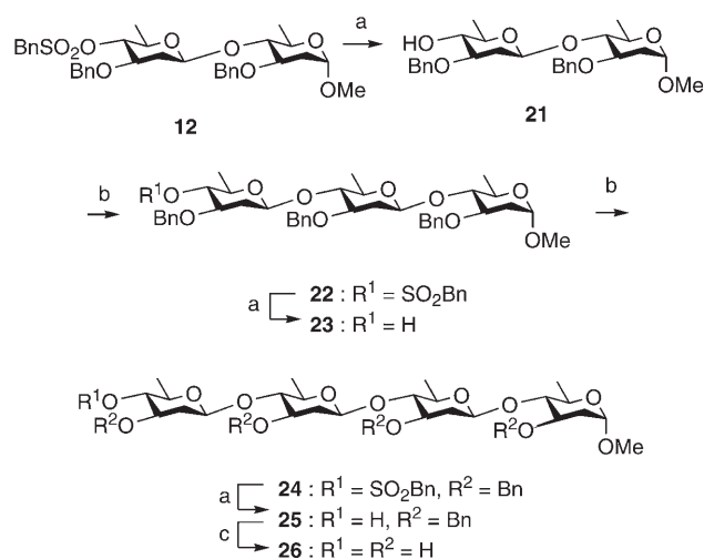
Scheme 1. Synthesis of \beta -(1 \rightarrow 4)-tetraolivoside 26 . Reagents and conditions: a) NaNH_2 , DMF, microwaves, 84% for 21 , 76% for 23 , 68% for 25 ; b) 1a (1.5 equiv), I_2 , Et_3SiH , toluene, -94^\circ C , 93%, \beta/\alpha 93:7 for 22 , 80%, \beta/\alpha 93:7 for 24 ; c) H_2 (1 atm), Pd(OH)_2 , EtOAc/MeOH (1:1), 72%.
